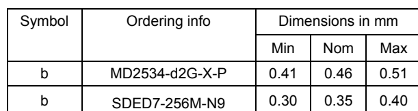
Figure 35: Mechanical Dimensions 9x12 FBGA Package
